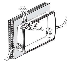
Standard-feature rubber cable gland
