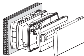
Recessed installation
